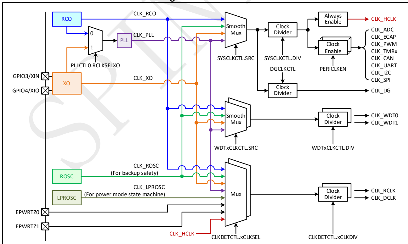
Figure 1-3: Clock tree
