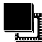
QFN48 (7 x 7 mm, 0.5mm pitch) QFN56 (8 x 8 mm, 0.5mm pitch)
