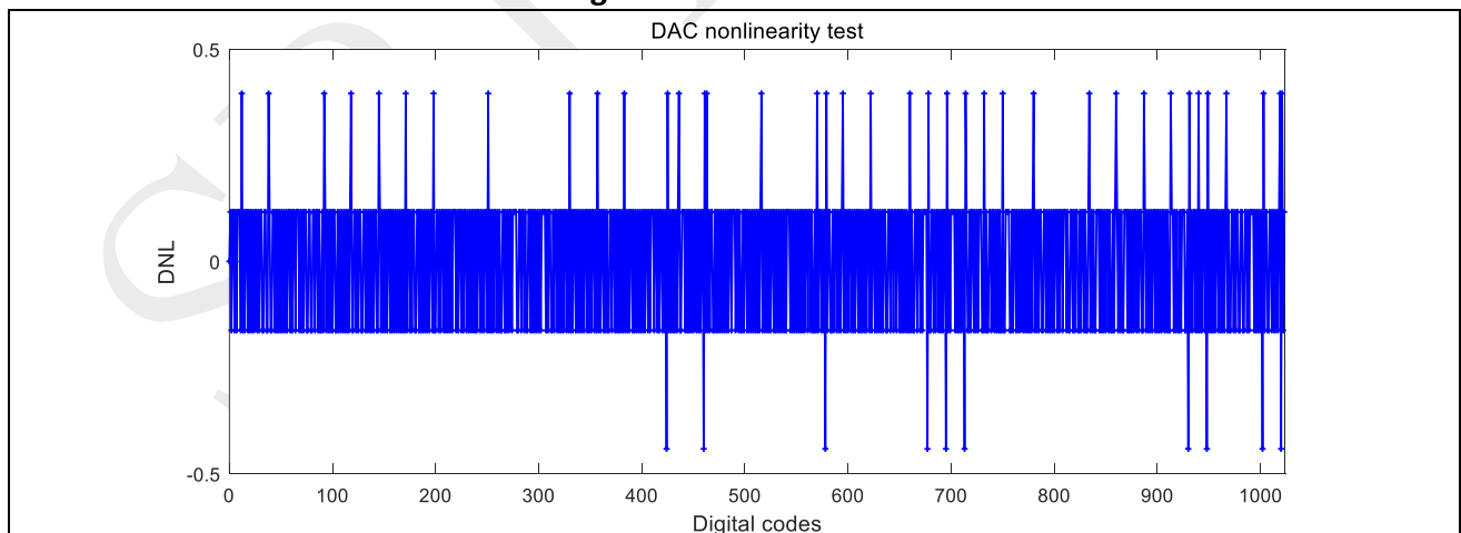
Figure 5-12: DNL curve
