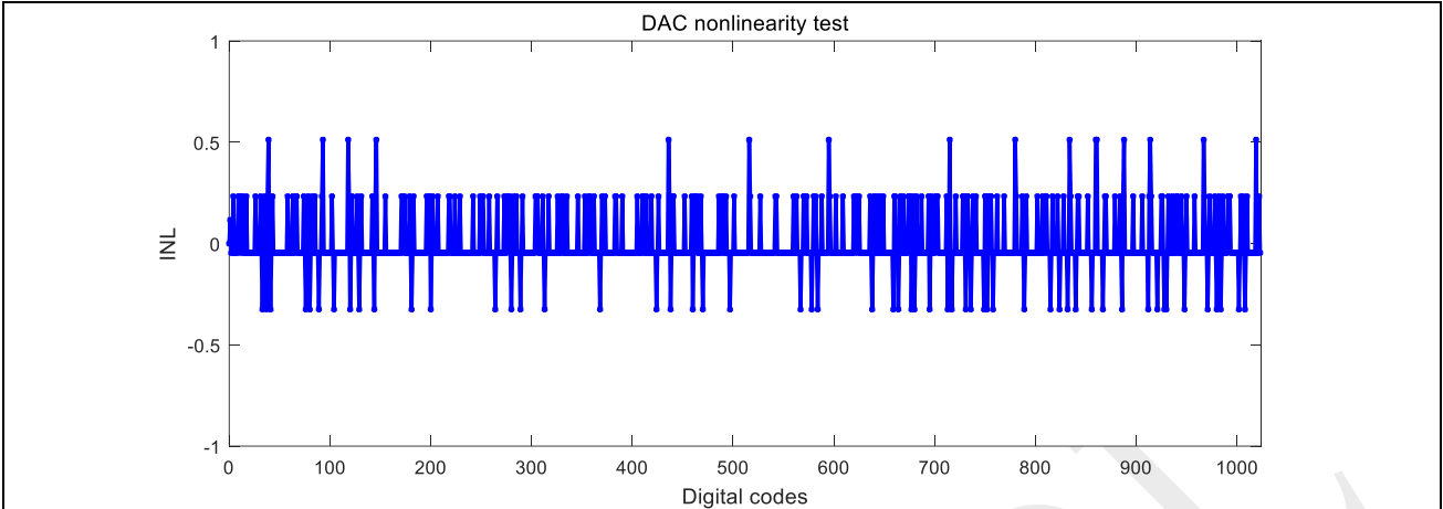
Figure 5-13: INL curve
