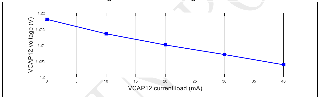
Figure 5-17: VCAP12 load regulation
