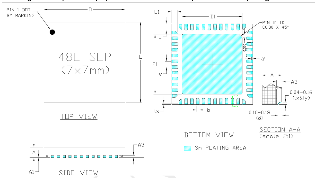
Figure 6-1: QFN48 - 48 pin, 7 x 7 mm wettable flank quad flat no-lead package outline
